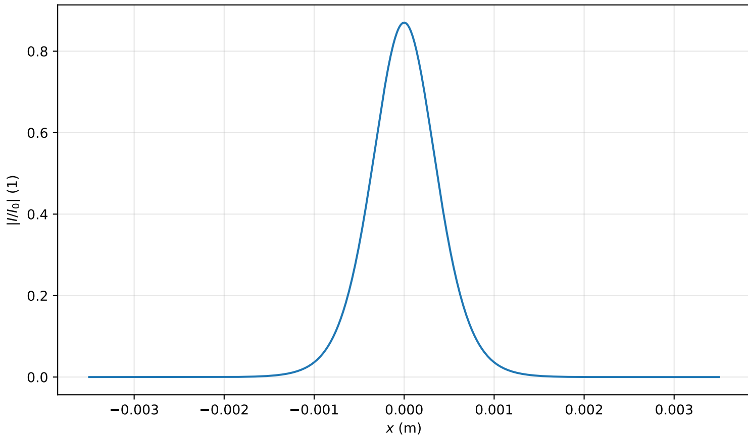
Intensity profile I(x, y = 0, z = 1.831m)/I_0 , P_{in}=0.5P_{cr} , artificial time
